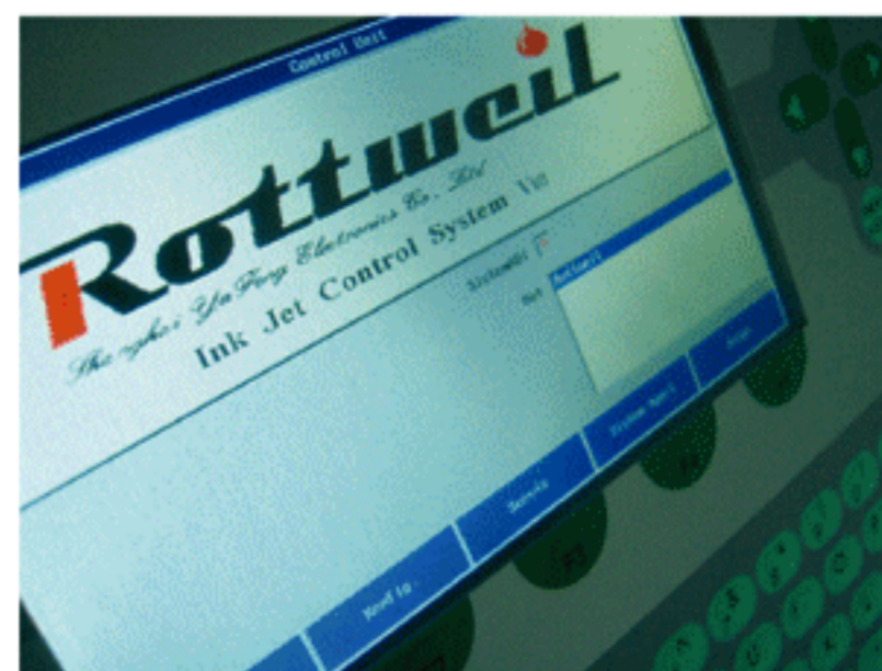
Linux System
